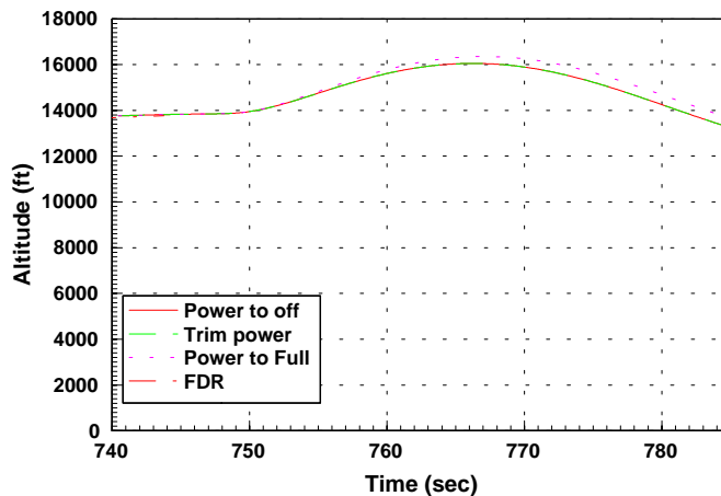
TWA 800 Main Wreckage Simulation Longitudinal Motion Only
